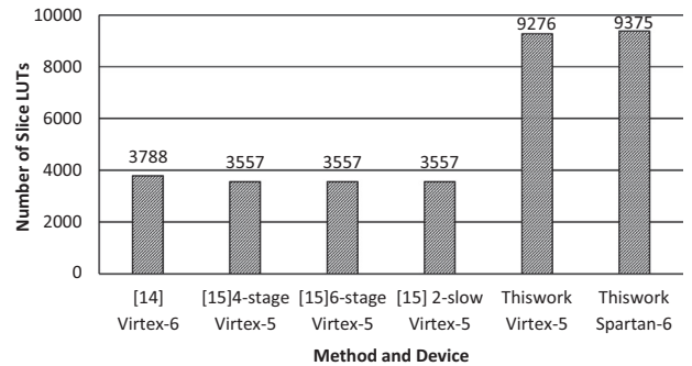
Figure 5 Slice LUTs comparison between existing and proposed work.
