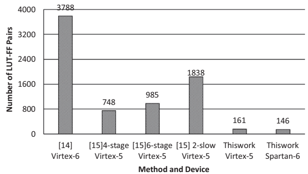
Figure 6 LUT-FF comparison between existing and proposed work.
