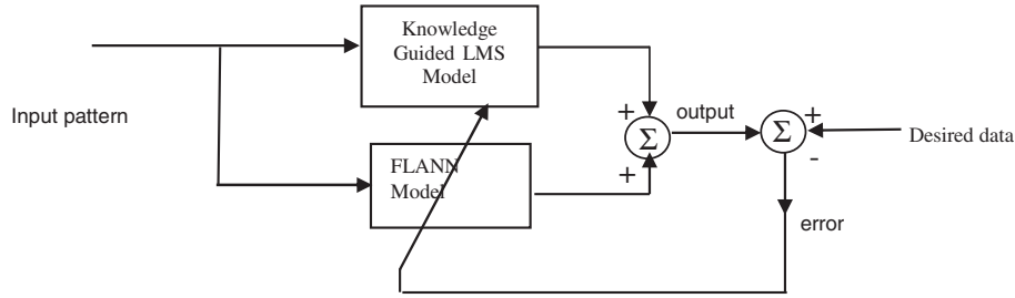
Figure 1 Knowledge guided ANN forecasting model.
