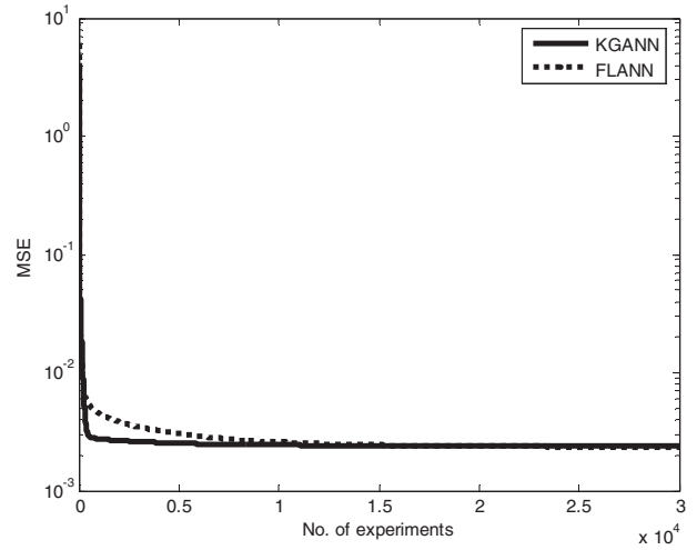
Figure 5b Comparison of convergence characteristics of knowledge base and FLANN models of Pound conversion for twelve months ahead of prediction.
