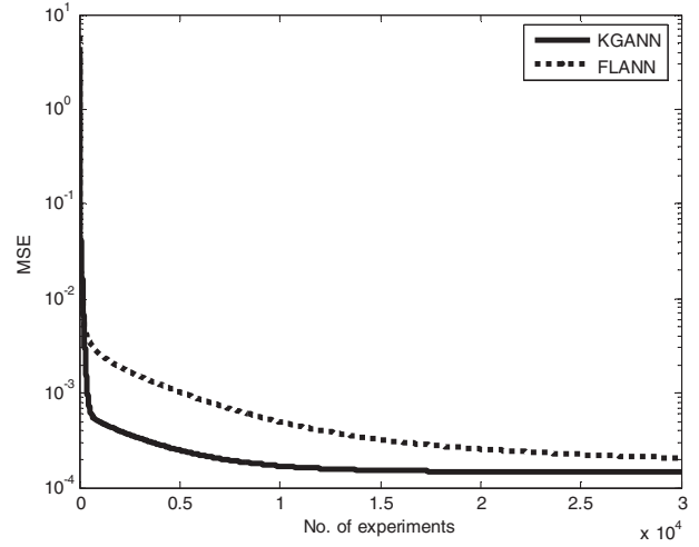
Figure 5a Comparison of convergence characteristics of knowledge base and FLANN models of Pound conversion for one month ahead of prediction.
